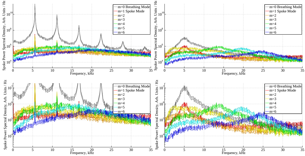
Figure 7. Selected 2D DFT power spectra observed in operating mode transitions at 105V, 10 mg/s. Top left, high-current mode operation with a dominant m = 0 breathing mode oscillation; top right, the low-current mode showing a much more quiescent oscillation spectra. Bottom, enlarged images of both spectra show the shift in spoke mode structure from broadband frequency structures in the high-current mode to clearly peaked structures in the low-current mode, indicating the formation of more stable and coherent spokes. This transition from an exaggerated breathing mode with decoherent spokes to a quiescent discharge with more stabilized spokes corresponds to a reduction in backstreaming electron current and an improvement in thruster operating efficiency.
