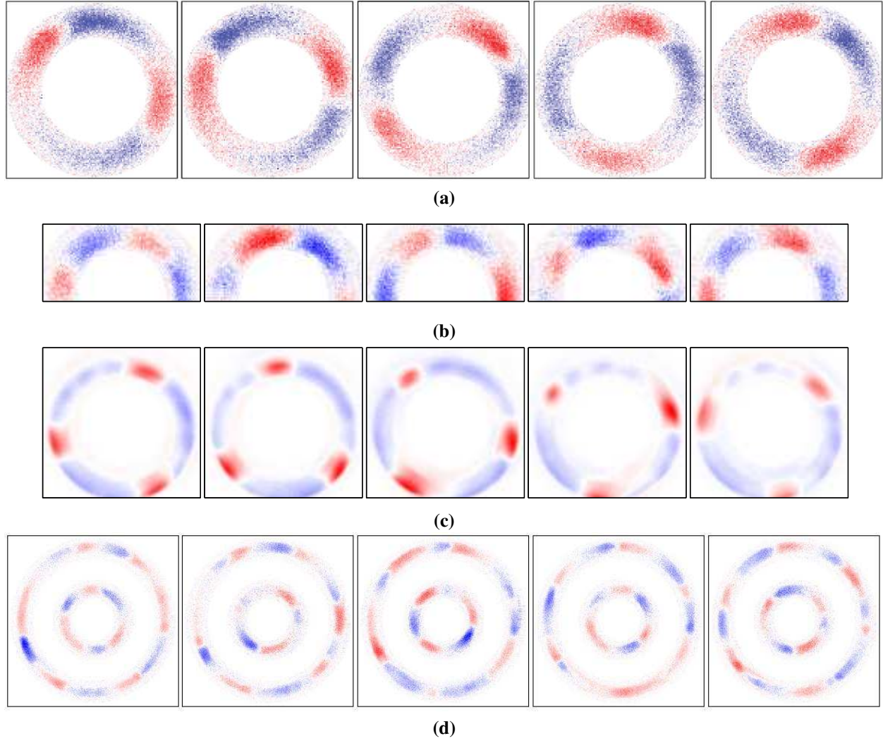
Figure 2. Postprocessed video frames showing rotating spokes in several Hall thrusters: (a) the H6 operating at 300 V and 10 A with a m = 2 spoke mode, imaged at 27000 fps; (b) the NASA 173Mv1 operating at 300 V and 7 A with a m = 3 spoke mode, imaged at 45000 fps (only part of the thruster was imaged to achieve a higher framerate with the 1024PCI camera); (c) the Helicon Hall thruster (HHT) operating at 200 V and 23.5 A with a very clearly delineated m = 3 spoke mode, imaged at 162,500 fps with only every fourth image shown; (d) the X2 dual nested channel Hall thruster operating at 150V, 6.6 A on the inner channel and 16.8 A on the outer channel, with an m = 3 mode on the inner channel and a m = 5 - 6 mode on the outer channel. The spokes counter-rotate in the X2 due to reversed magnetic field direction between the channels.
