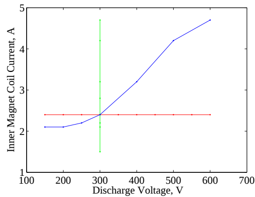
Figure 3. Parameter space for H6 operating regime investigation of rotating spokes.
