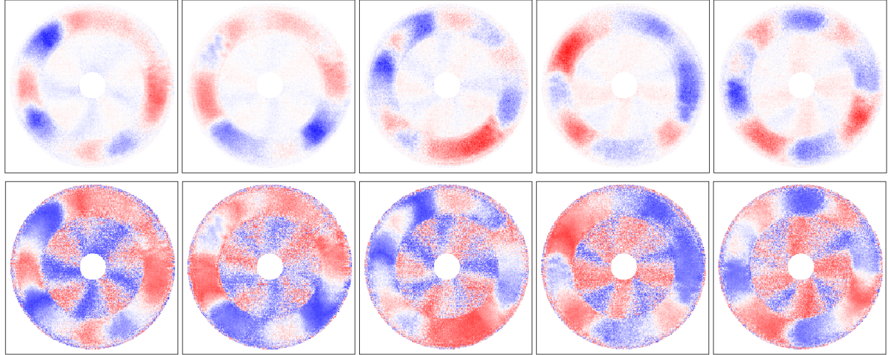
Figure 8. Top, a postprocessed set of still frames show the H6 operating at 300V, 10A with the segmented anode, imaged at 87.5 kfps. Bottom, the same frames are plotted but showing the normalized fluctuation amplitude in Eqn. 2. This rescaling of the visible signal based on the peak-to-peak oscillation amplitude of each pixel makes the radial extent of the spoke structure visible even in the very dim regions over the inner pole, and show that the spokes can form a bridge between the cathode and the exit plane across the near field. Note that the central cathode is still cropped from both image series, since the bright cathode discharge saturates the camera sensor and oscillations are not discernible over the saturated pixel signal.
