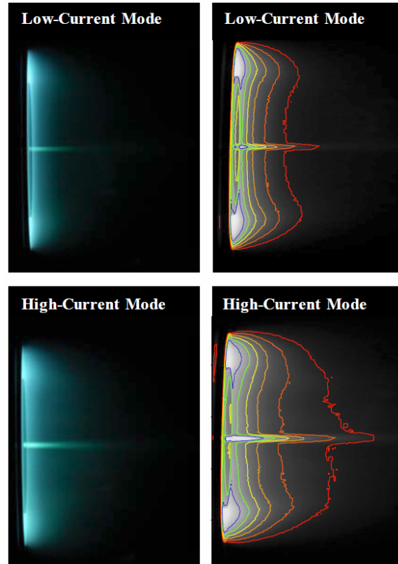
Figure 6. Figure and caption reprinted from Brown 23 : Photographs of the [H6] 6-kW Hall thruster jet-mode plume structure for the low-current mode (top left) and high-current mode (bottom left) during 105-V, 20-mg/s operation. Contours of constant image intensity are shown for the low-current mode (top right) and the high-current mode (bottom right). Photos were taken with identical settings on a tripod mounted Nikon D200 DSLR using a 70-mm lens with manual focus at F/5, ISO-400, and exposure time of 1/2000 sec.
